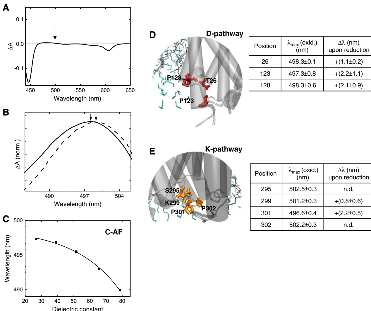
Fig. 7. (A) Difference spectra of oxidized minus reduced enzyme. (B) Fluorescein difference spectra (labeled minus unlabeled protein) in the oxidized (solid) and reduced (dashed) state of CS-T26C-AF. (C) The wavelengths of the absorption maxima of cysteine-bound amido fluorescein (C-AF) in 150 mM KCl and in water/ethanol-mixtures at pH 9 plotted against the dielectric constants. (D) Close up of amino acids in CcO exchanged to cysteine at the entrance of the D-pathway. Grey: protein, red: amino acids exchanged to cysteine, cyan: water molecules. The wavelength of the absorption maximum ( \lambda_{\text{max}} ) of the cysteine bound fluorescein in the oxidized state at pH 9, as well as the \lambda_{\text{max}} shift upon reduction of the solubilized enzyme are determined. (E) Close up of amino acids in CcO exchanged to cysteine at the entrance of the K-pathway. Grey: protein, yellow: amino acids exchanged to cysteine, cyan: water molecules. The wavelength of the absorption maximum ( \lambda_{\text{max}} ) of the cysteine bound fluorescein in the oxidized state at pH 9, as well as the \lambda_{\text{max}} shift upon reduction of the solubilized enzyme are determined. The \lambda_{\text{max}} -shift values are the mean from 2 or 3 independent measurements. SEM is given.
